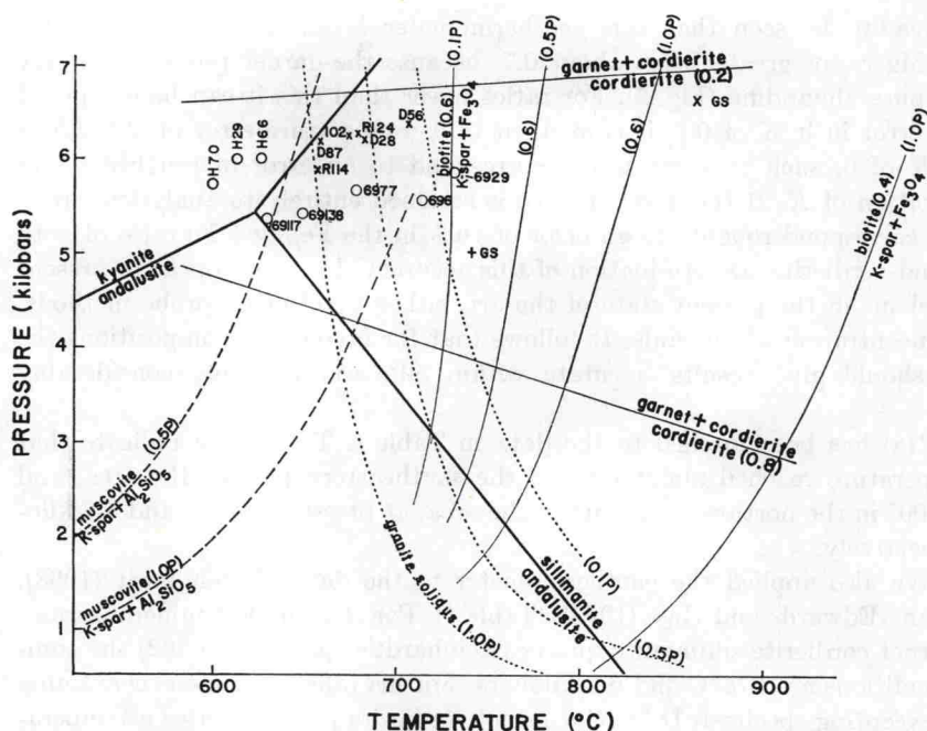
Fig. 3. PT projection of garnet-cordierite equilibrium and other relevant experimental data. The figures in brackets on the experimental univariant curves give the Fe/Fe+Mg ratio of the starting materials, while the figures at the end of the curves (e.g. 0.5 P) give the water pressure as a fraction of total pressure. The biotite breakdown curve is calculated for the quartz-fayalite magnetite buffer. Numbered and lettered points are those shown in Tables 1 and 4. The two points labelled GS represent the migmatitic and nonmigmatitic garnet-cordierite gneisses analyzed by Gable and Sim (1969). Specimen 69117 contains andalusite plus sillimanite, while all others contain sillimanite, although specimens H 70, H 29, and H 66 appear to fall in the Kyanite field.
